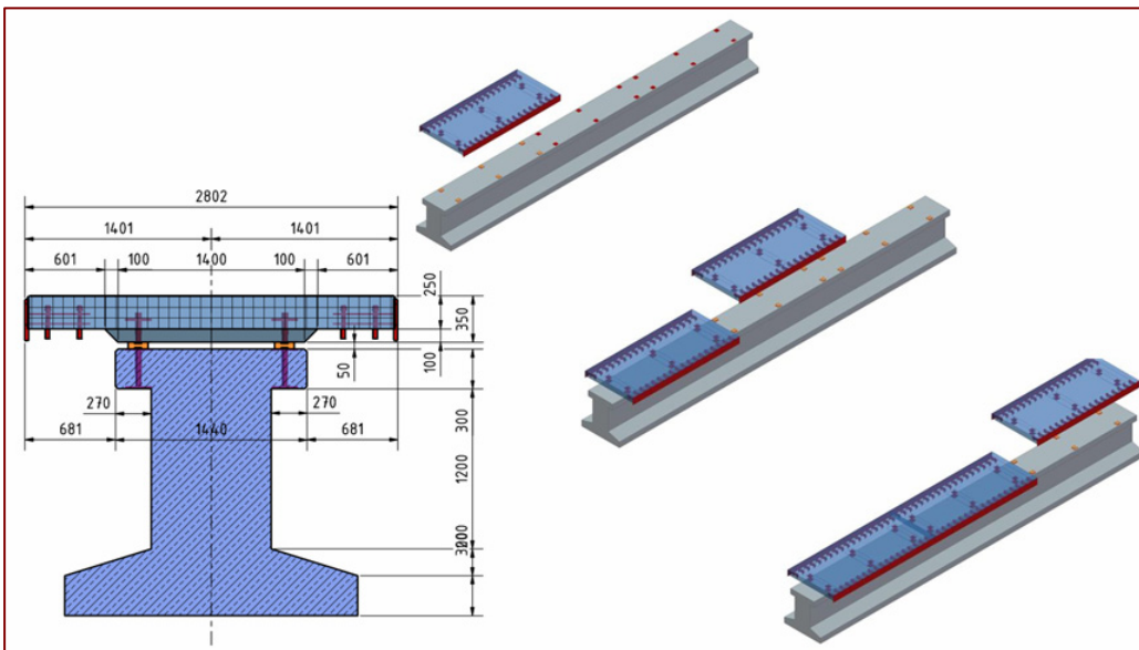
Figure 3: Track of Type III, Züblin design (Source Züblin)
