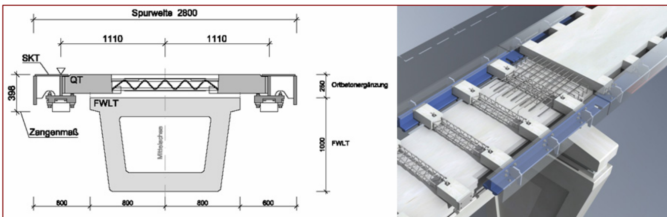
Figure 2: Track of Type II, BGmU design (Source: BGmU)
