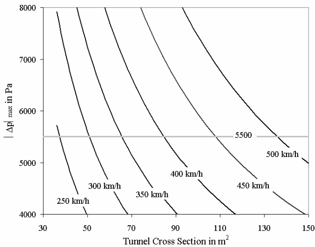
Figure 3: Maximum pressure variation |\Delta p|_{\max} acting on a 12.4 \text{ m}^2 -train in a tunnel with respect to tunnel cross-section and train speed (single-track tunnel, no pressure waves of other trains, no shafts, train length 100m, “critical” tunnel length).
