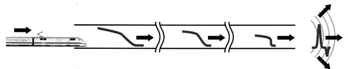
Figure 1: Illustration of development of micro-pressure waves.
