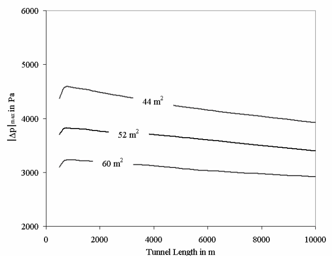
Figure 2: Maximum pressure variation |\Delta p|_{\max} acting on a 12.4 m 2 -train in a tunnel with respect to tunnel length and tunnel cross-section (single-track tunnel, no pressure waves of other trains, no shafts, train length 100m, train speed 250 km/h).
